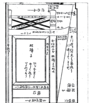
図1-4 脇障子笠木の禪墨
