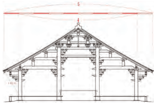
図3-4 浄土寺浄土堂の軒比率と禪墨
