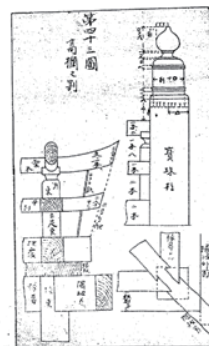
図1-3 勾欄の禪墨
