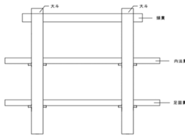
(c) 試験体III
