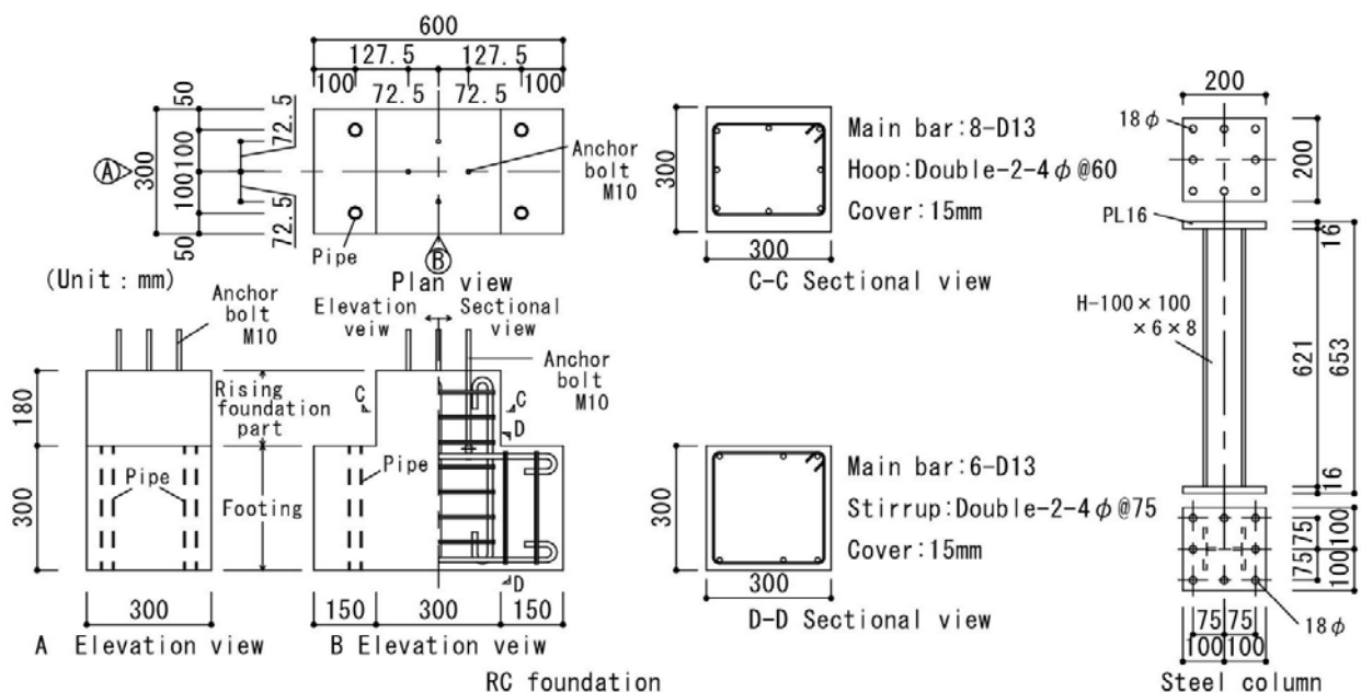
Fig. 1 RC foundation Shape dimensions and reinforcement arrangement ,Steel column Shape
